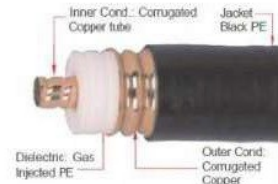
1-5/8" Hansen Feeder Cable
