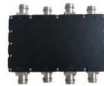
4 In 4 Out 698- 3800MHz 50 Ohm Combiner
