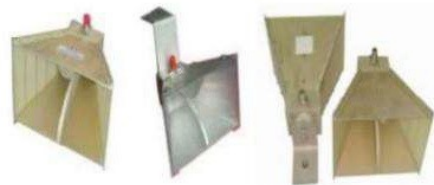
Wideband Dual-ridged Horn Antenna
