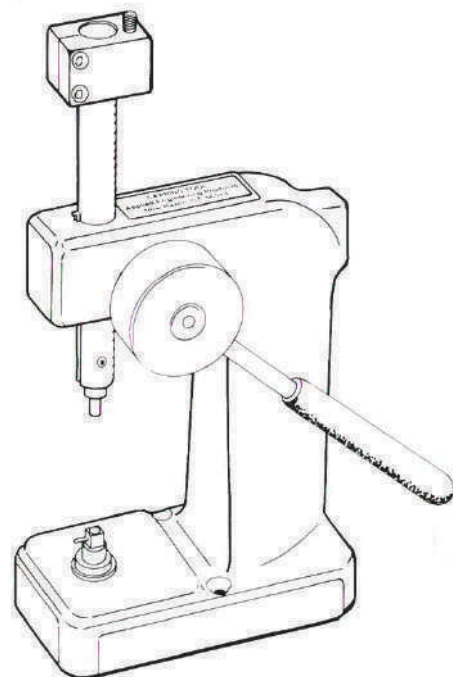
Capping tool for right angle connectors.
