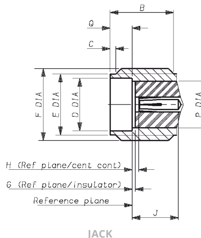
JACK
