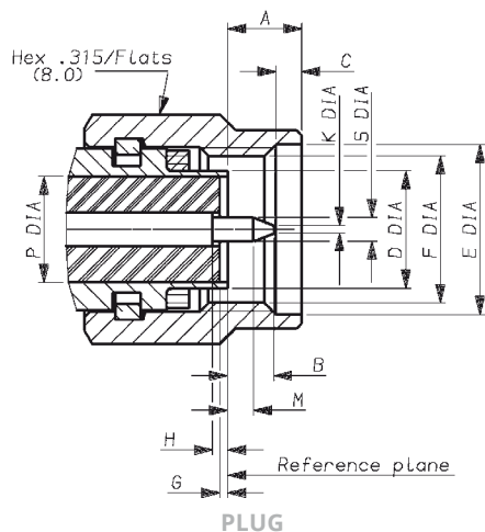
PLUG
