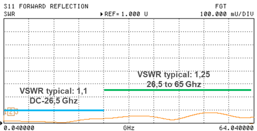
Legend: VSWR <1.10 up to 64 GHz
