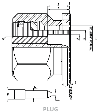
PLUG
