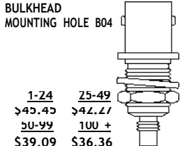
Model No. ST9108 BNC FEMALE TO SMC JACK BULKHEAD MOUNTING HOLE B04
