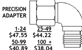
Model No. ST9641 SMA MALE TO SMA FEMALE RIGHT ANGLE MAX VSWR 1.35:1 @ 27 GHz
