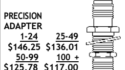
Model No. ST9652 2.4mm FEMALE TO 3.5mm FEMALE MAX VSWR 1.25:1 @ 34 GHz
