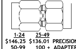
Model No. ST9649 2.4mm MALE TO 3.5mm MALE MAX VSWR 1.25:1 @ 34 GHz
