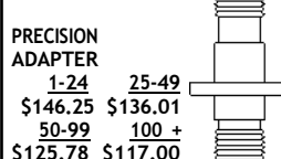
Model No. ST9653 2.4mm MALE TO SMA MALE MAX VSWR 1.20:1 @ 26.5 GHz
