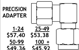
Model No. ST9642 SMA MALE TO SMA MALE RIGHT ANGLE MAX VSWR 1.35:1 @ 27 GHz
