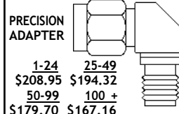
Model No. ST9644 2.92mm MALE TO 2.92mm FEMALE RIGHT ANGLE MAX VSWR 1.40:1 @ 40 GHz
