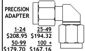
Model No. ST9645 2.92mm MALE TO 2.92mm MALE RIGHT ANGLE MAX VSWR 1.40:1 @ 40 GHz
