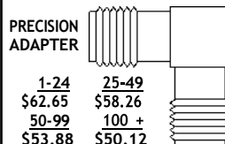
Model No. ST9643 SMA FEMALE TO SMA FEMALE RIGHT ANGLE MAX VSWR 1.35:1 @ 27 GHz
