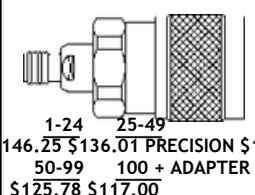
Model No. ST9663 2.92mm FEMALE TO N MALE MAX VSWR 1.15:1 @ 18 GHz
