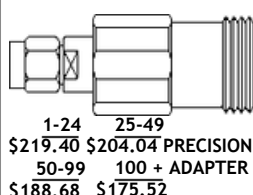
Model No. ST9662 2.92mm MALE TO N FEMALE MAX VSWR 1.15:1 @ 18 GHz
