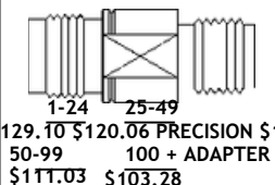
Model No. ST9657 3.5mm MALE TO 2.92mm MALE MAX VSWR 1.25:1 @ 34 GHz
