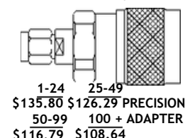
Model No. ST9661 2.92mm MALE TO N MALE MAX VSWR 1.15:1 @ 18 GHz
