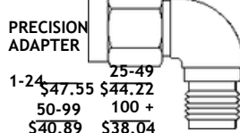
Model No. ST9646 2.92mm FEMALE TO 2.92mm FEMALE, RIGHT ANGLE MAX VSWR 1.40:1 @ 40 GHz
