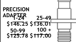
Model No. ST9653 2.4mm MALE TO SMA MALE MAX VSWR 1.20:1 @ 26.5 GHz
