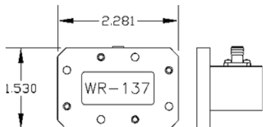
WAVEGUIDE TO N FEMALE
