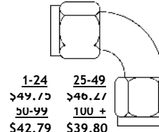
Model No. ST9273 SMA MALE TO SMA MALE RADIUS RIGHT ANGLE
