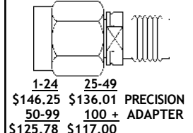
Model No. ST9655 2.4mm MALE TO SMA FEMALE MAX VSWR 1.20:1 @ 26.5 GHz
