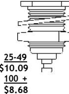
Model No. ST4879 MCX PLUG, RIGHT ANGLE CRIMP ATTACHMENT FOR RG188-DS & RG316-DS
