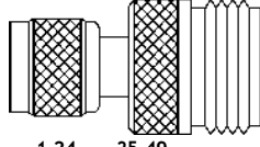
Model No. ST9183 MINI UHF MALE TO N FEMALE
