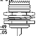
Model No. ST44060 UHF FEMALE BULKHEAD, REAR MOUNT, SOLDER CUP CONTACT MOUNTING HOLE B12
