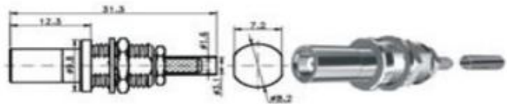
Straight Bulkhead Cable Plug, M06
